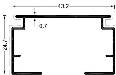
COD 5.33 G=0.25 kg/m
