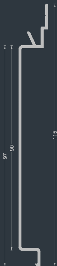
COD 6.26 G = 0.46kg/m P = 283mm
