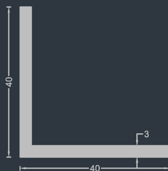
COD 12.7 G = 0.63kg/m P = 160mm
