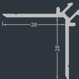
COD 6.47 G = 0.30kg/m P = 150mm
