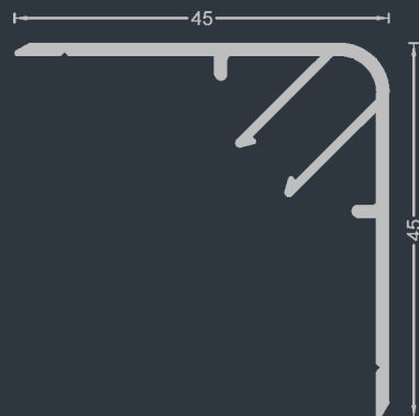
COD 6.46 G = 0.48kg/m P = 246mm
